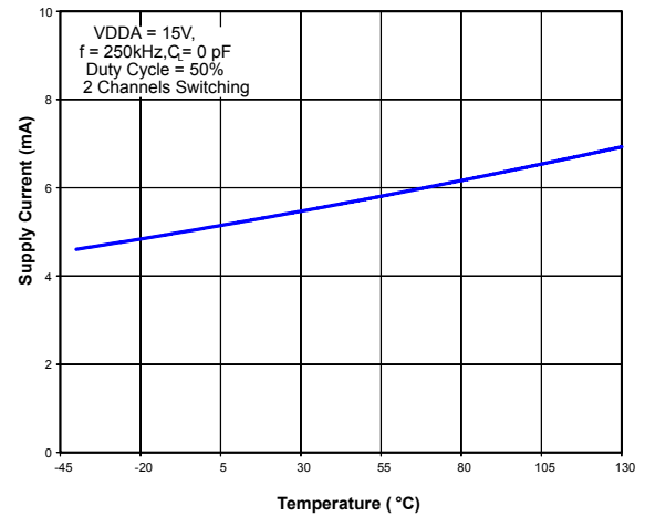
Figure 3.23. Supply Current vs. Temperature
