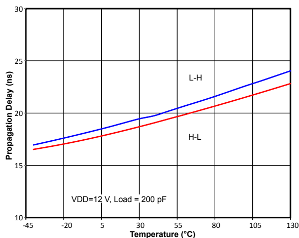
Figure 3.10. Propagation Delay vs. Temperature
