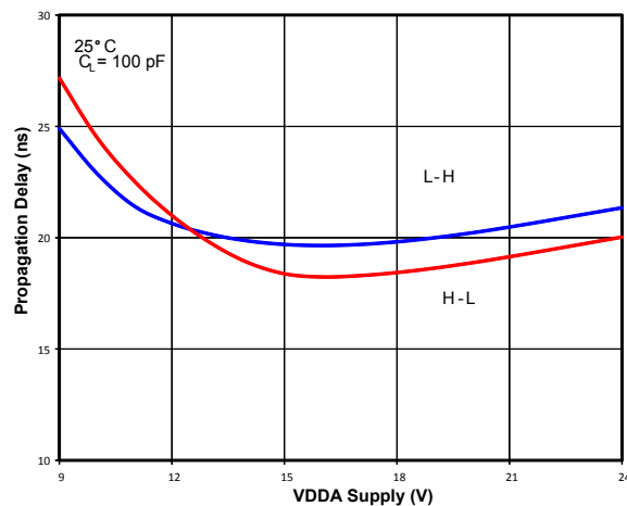
Figure 3.19. Propagation Delay vs. Supply Voltage
