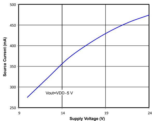
Figure 3.14. Output Source Current vs. Supply Voltage
