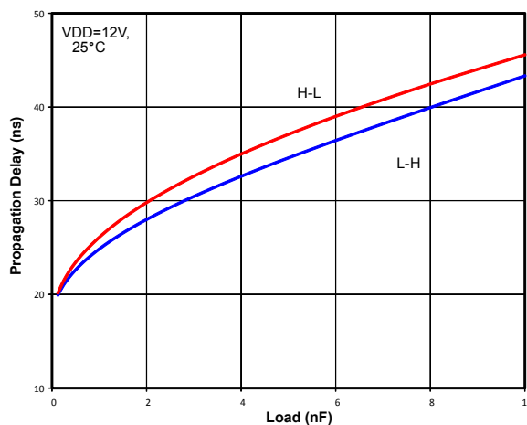
Figure 3.21. Propagation Delay vs. Load
