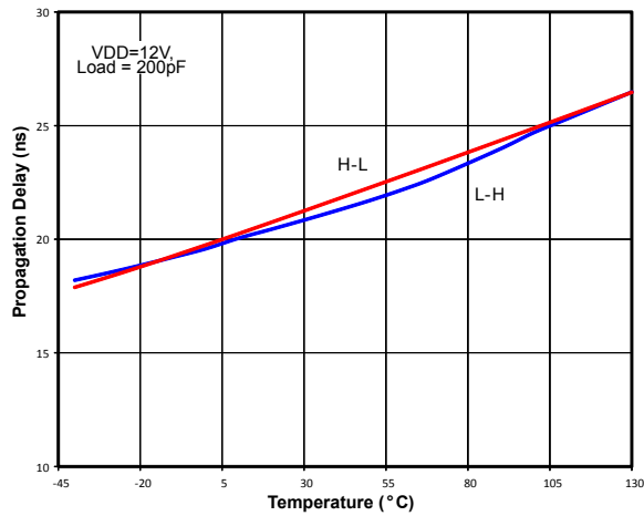
Figure 3.22. Propagation Delay vs. Temperature
