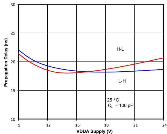
Figure 3.7. Propagation Delay vs. Supply Voltage
